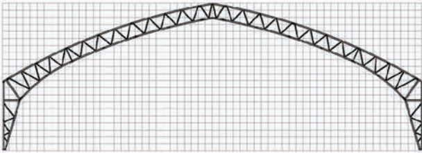
120' Pinnacle™ with 19' Leg
